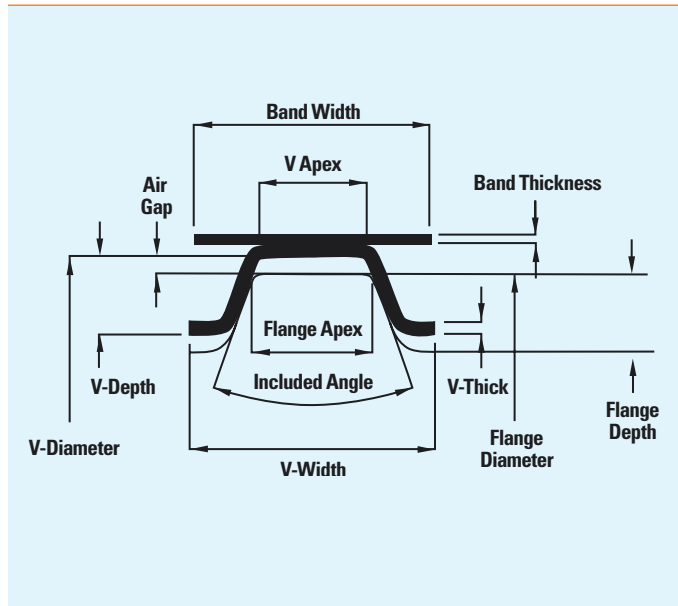
Typical V-insert Clamp
